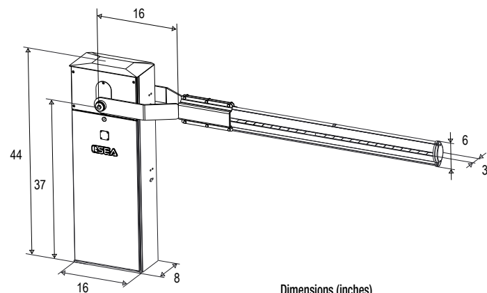
Dimensions (inches)
