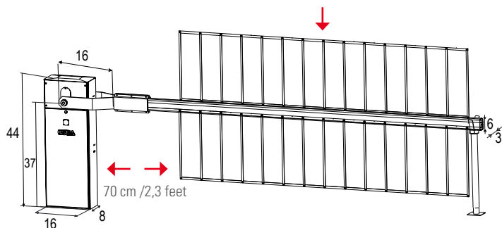
Dimensions (inches)
