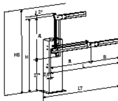
Articulated beam
