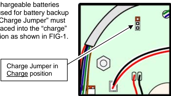
FIG-1: Charge Jumper Shown in Charge Position
