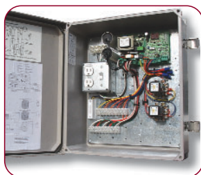
Model 455 D control panel in 14 in. x 16 in. enclosure (optional).
