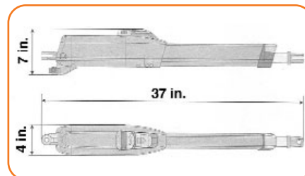
Model 415 dimensions
