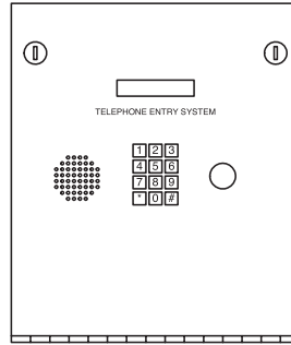
1803 Flush 12" W x 13.25" H x 3" D 30.4cm W x 33.65cm H x 7.62cm D
